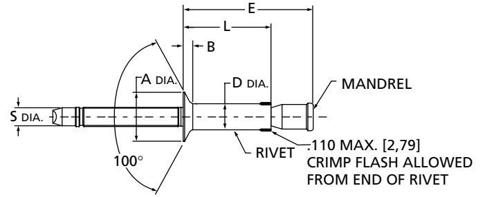
Countersunk Head
