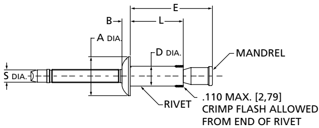
Protruding Head
